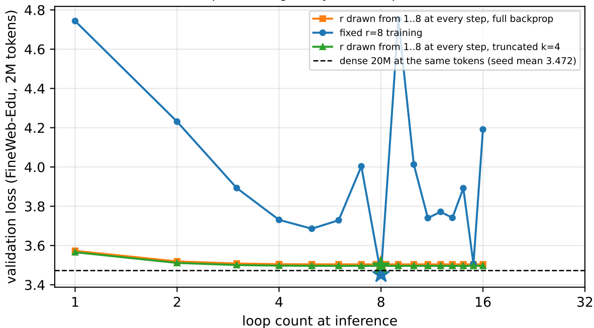
20M middle block, 32N-token trunk checkpoints: random loop-count training converges to a fixed point (robust to the loop count, no gain beyond \sim 4 loops); star = nominal r=8
