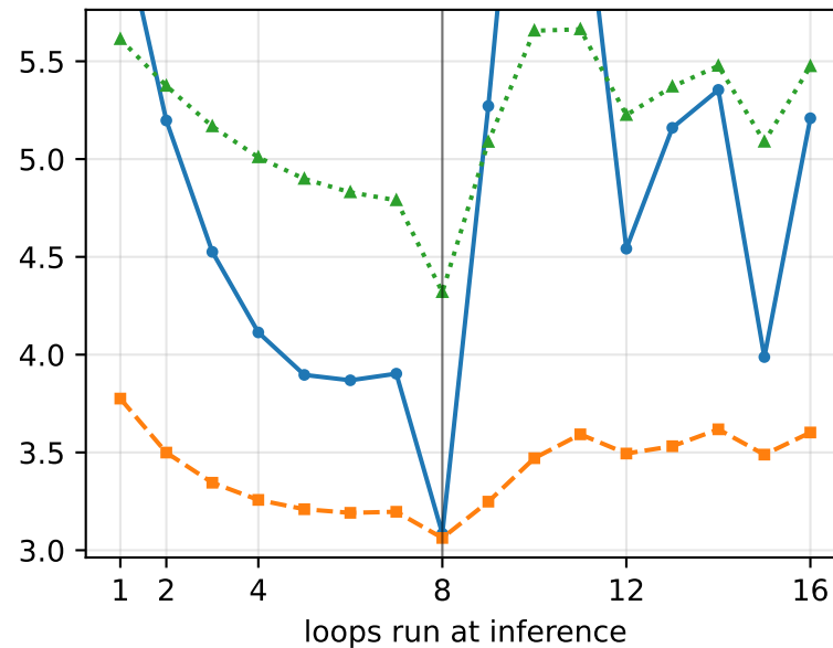
80M middle r8 (trained r=8)
