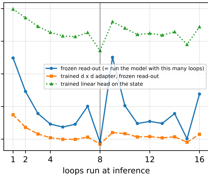
20M middle r8 (trained r=8)
