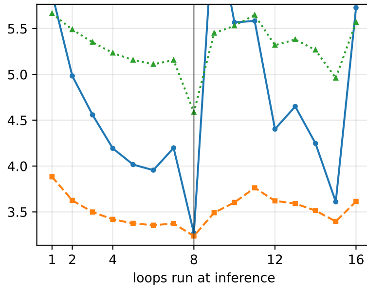
40M middle r8 (trained r=8)
