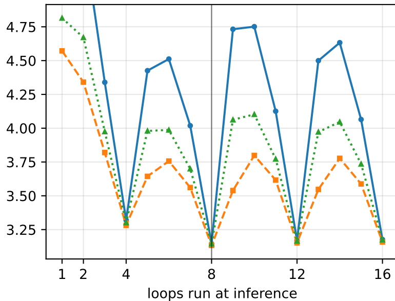
80M whole r8 k4 (trained r=8)
