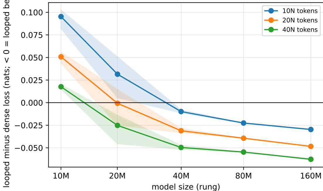
Middle block looped 4 times vs the dense model of the same size (seed mean; band = min-max over seeds; 3 seeds at 10M-40M, 1 at 80M, 2 at 160M)
