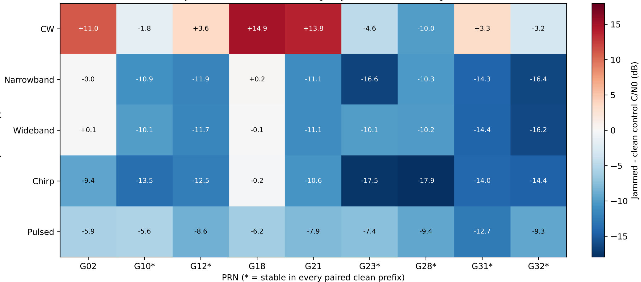
Matched jammer-interval C/N0 change by GNSS-SDR tracking channel
