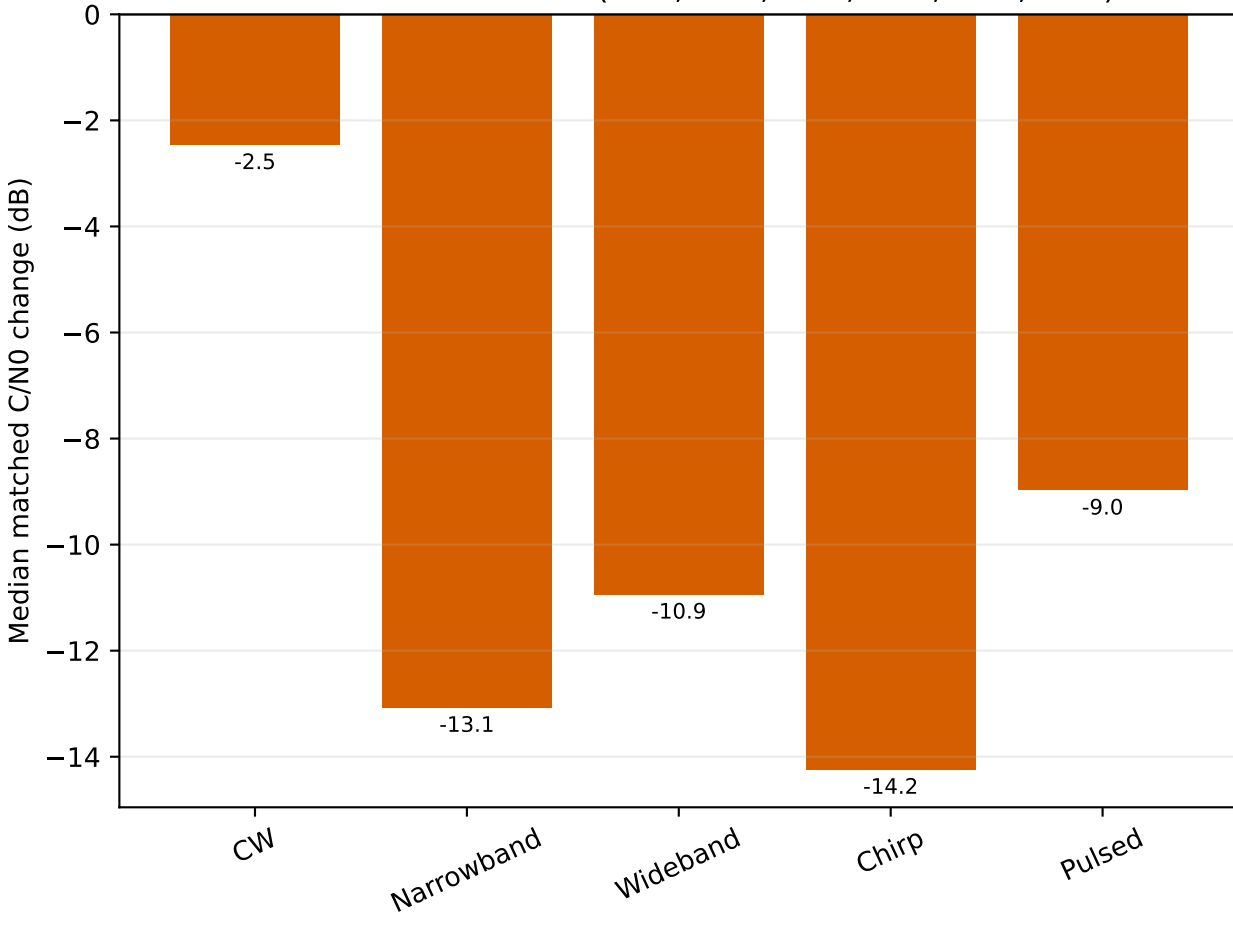
Common stable PRNs (G10, G12, G23, G28, G31, G32)
