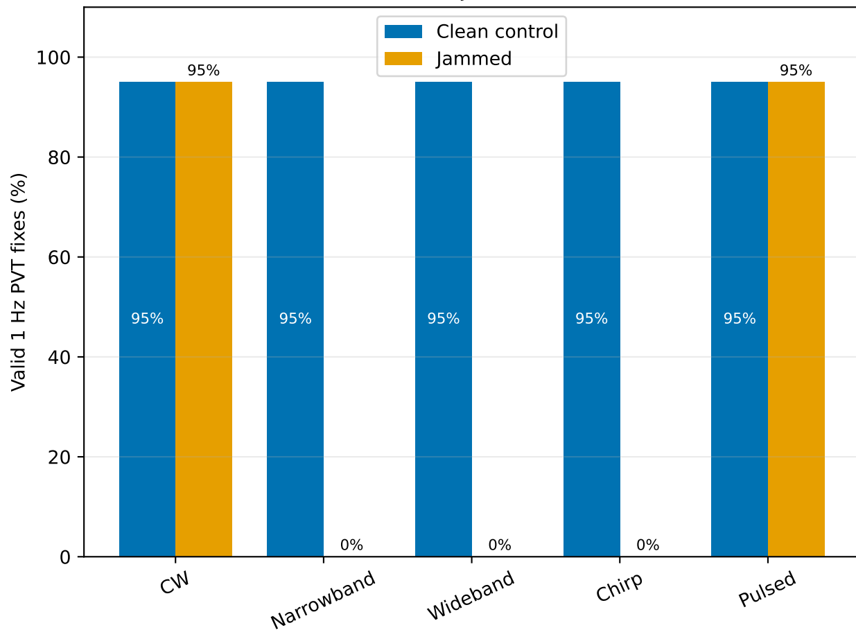
Matched 20 s jammer interval
