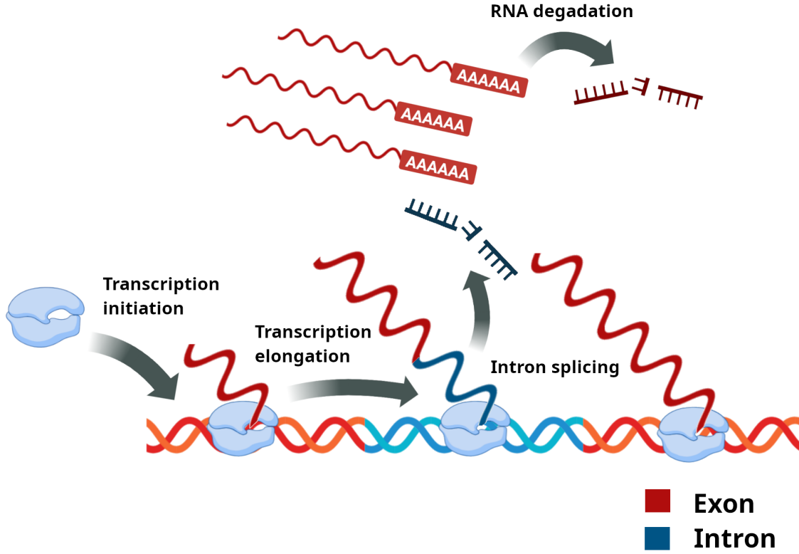
Figure 1: Schema of RNA metabolism.
