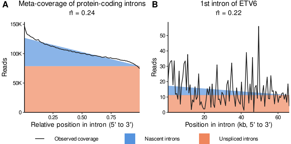
Figure 2: Read coverage of introns in K562 cells, using a total RNA-seq dataset of The ENCODE Project Consortium (2012) (accession ENCSR000AEL, two replicates pooled). The decrease of the coverage along the intron is clearly visible in the meta-coverage, while the coverage of a single intron is much noisier. In both panels, the black line is the observed coverage, and the shaded areas are the fitted mixture (8) of nascent introns (blue, linearly decreasing density (14)) and unspliced introns (orange, uniform density (12)); \hat{\pi} is the estimated fraction of reads originating from nascent introns. (A) Meta-coverage of all 166,239 protein-coding introns, containing 10.3 million reads in total. (B) Coverage of a single intron, the first intron of the ETV6 gene (66,426 bp, 1,432 reads). The coverage of every intron is rescaled to 100 equally sized bins, and normalized so that the binned values sum to the number of reads of that intron; one bin in panel B therefore spans 664 bp, and features narrower than a bin appear smoothed. The mixture is fitted here by maximum likelihood to the coverage shown. Our inference model also uses maximum likelihood, but parametrizes the mixture differently: there, \pi is not an independent parameter, but a function of several other parameters, which are all estimated jointly (see the section Inference Model), and it is always obtained for individual introns, rather than for a meta-coverage. The figure is therefore only an illustration of the coverage pattern, and does not show the output of our inference model.
