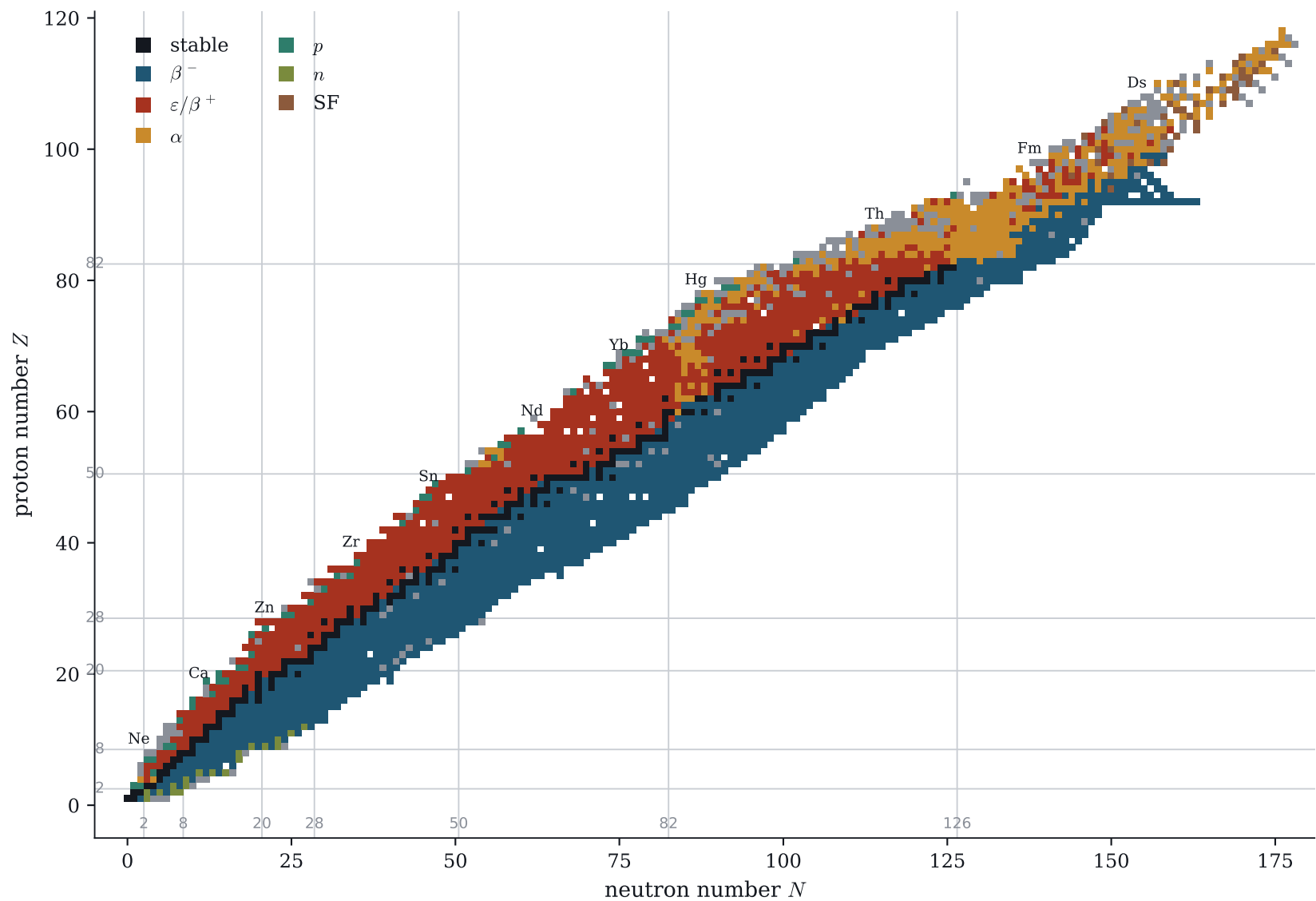
chart of nuclides (3371 nuclides, ENSDF)
