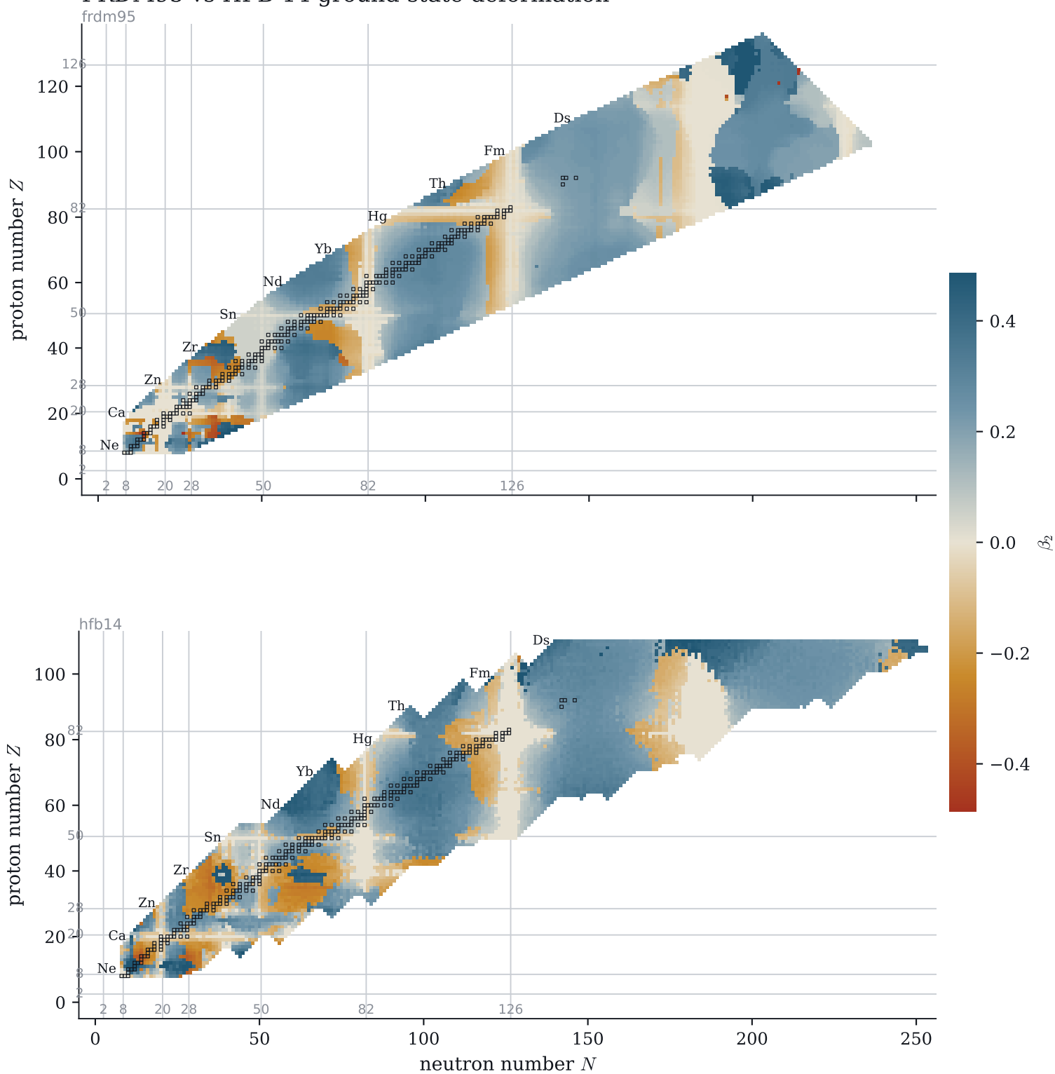
FRDM95 vs HFB-14 ground-state deformation
