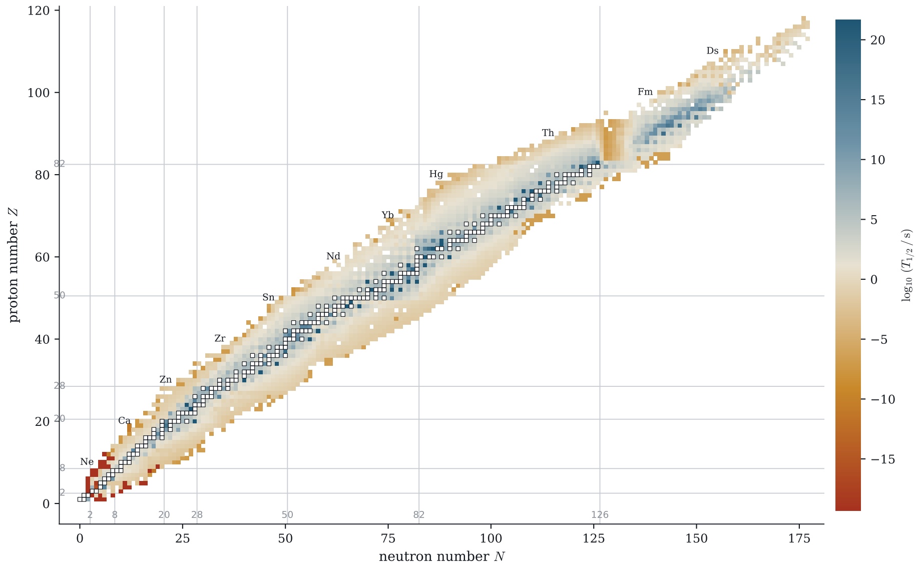
ground-state half-life
