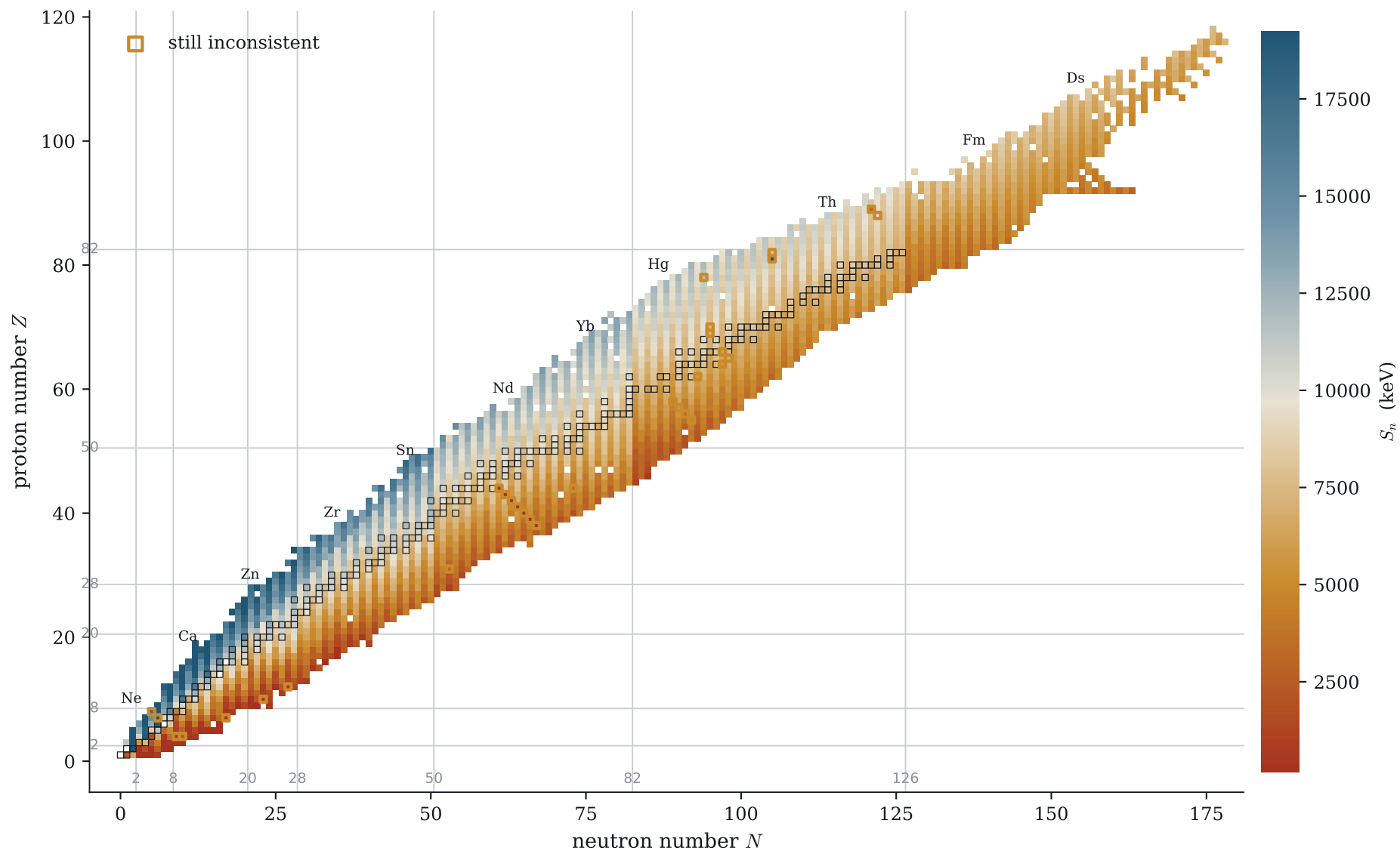
neutron separation energy after 19 verified repairs
