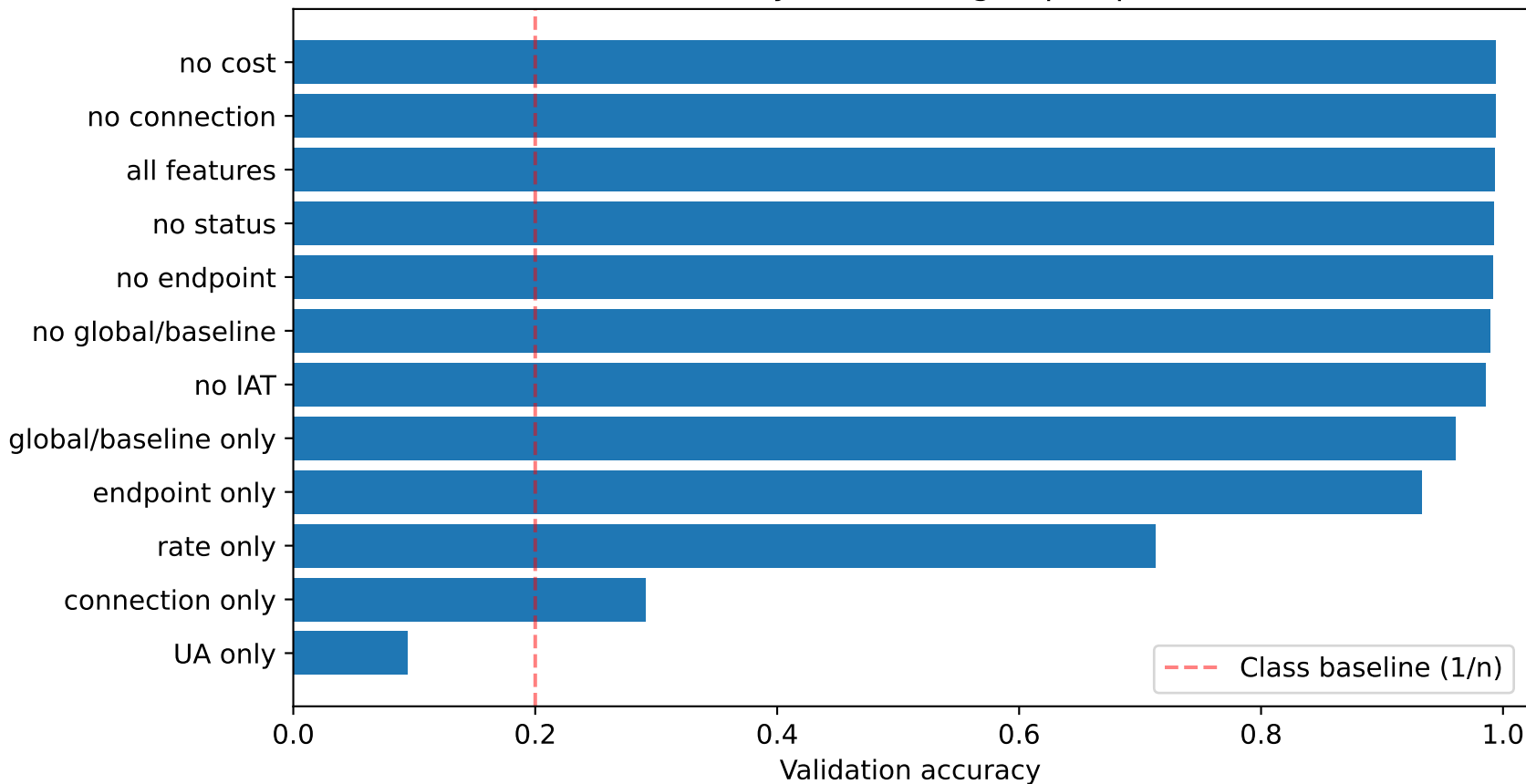
Ablation study — feature group importance
