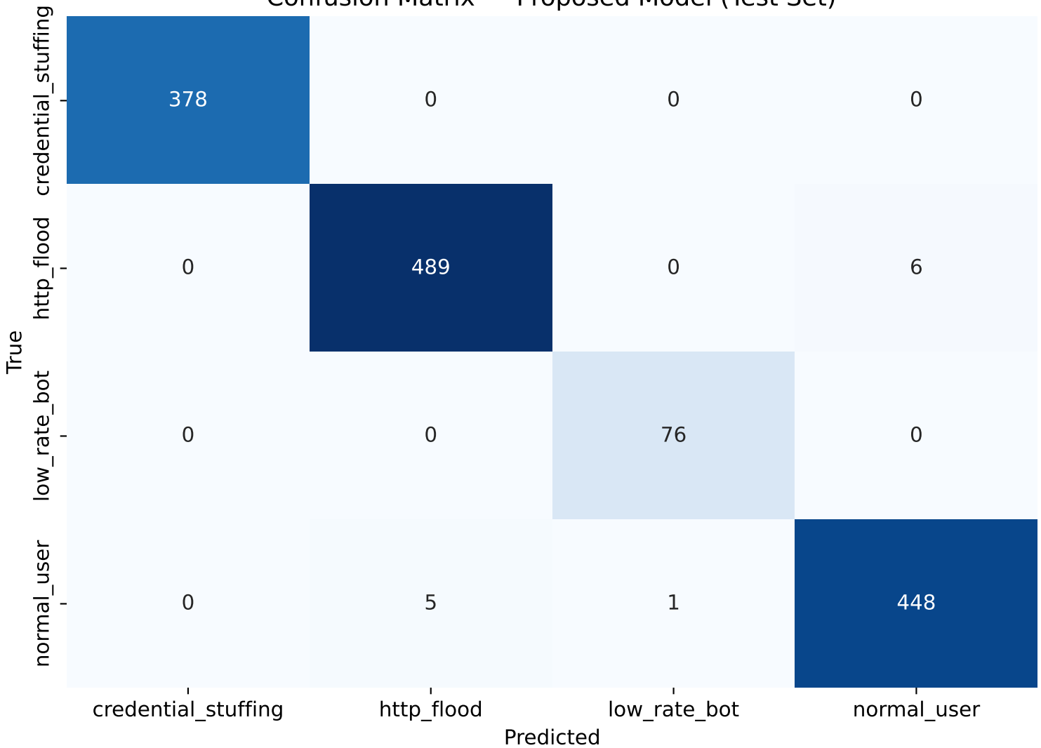
Confusion Matrix — Proposed Model (Test Set)
