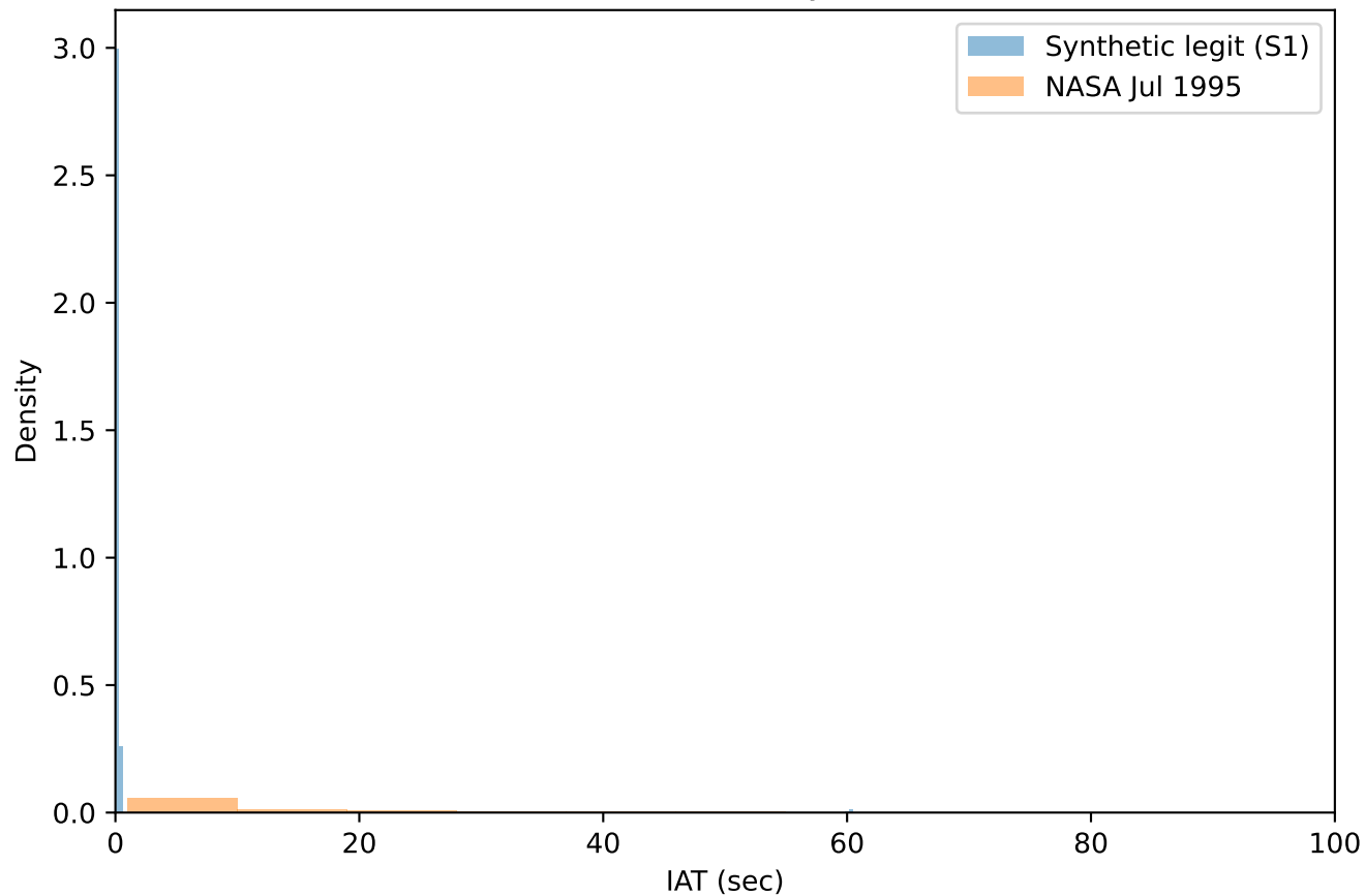
IAT distribution (linear) — synthetic vs NASA
