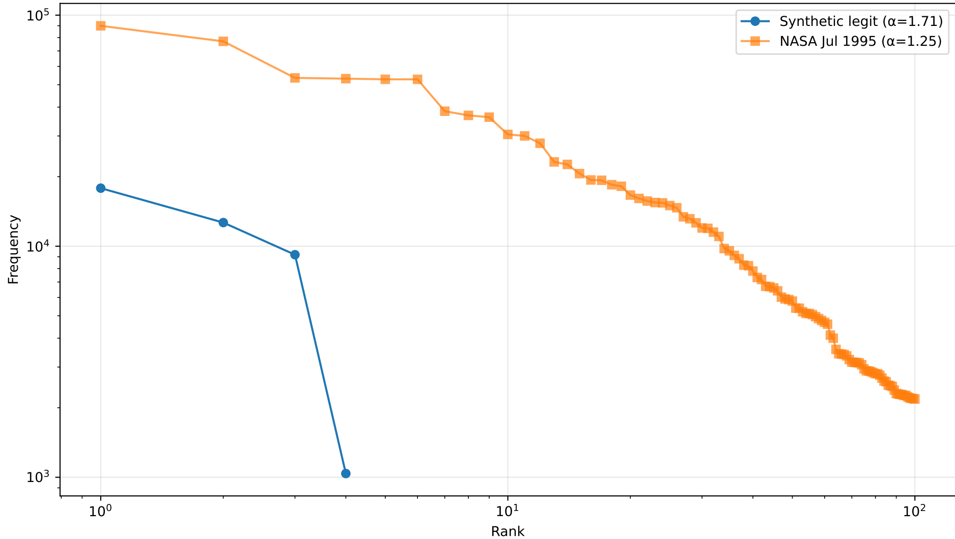
Endpoint popularity Zipf — synthetic vs NASA
