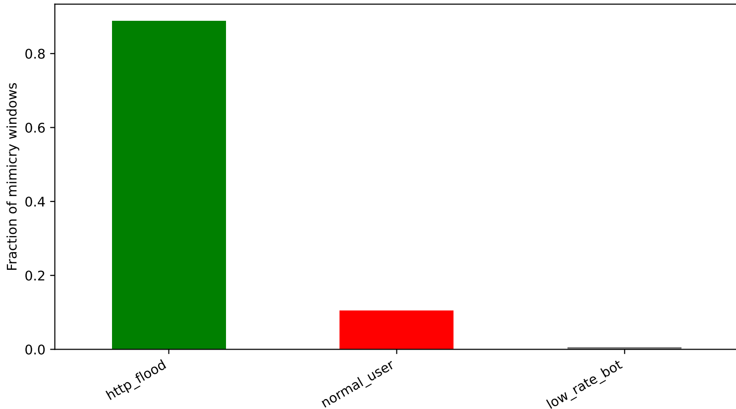
Mimicry holdout — Proposed model classification (green=correct flood, red=evasion as legit, gray=other)
