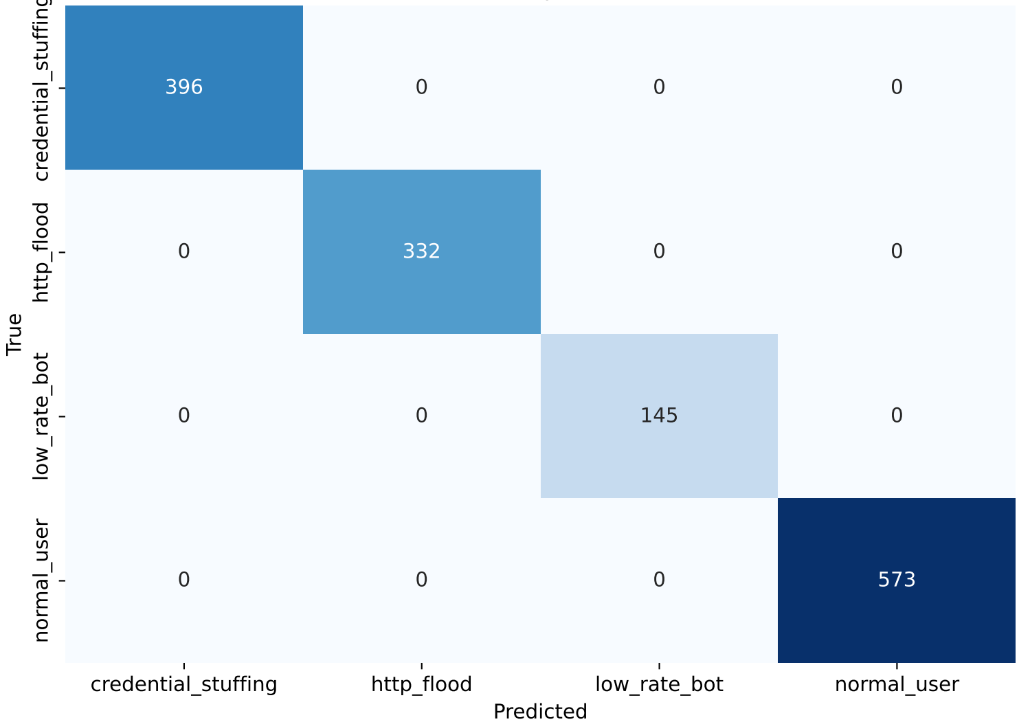
Confusion Matrix — Proposed Model (Test Set)
