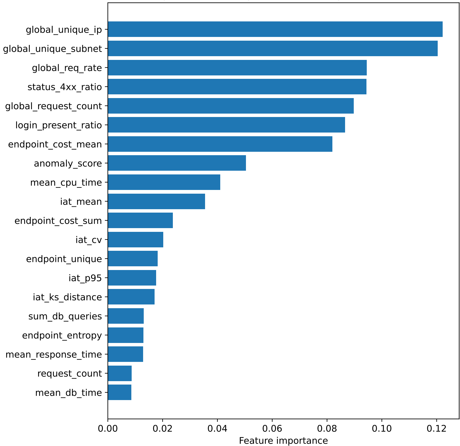
Top 20 feature importances — Proposed ISO+RF
