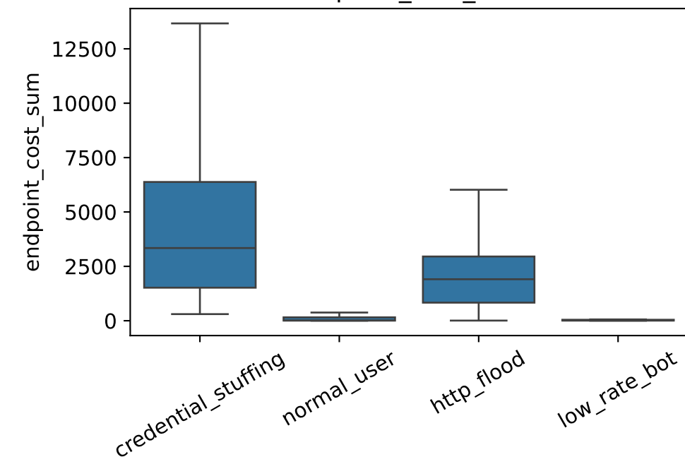
endpoint_cost_sum
