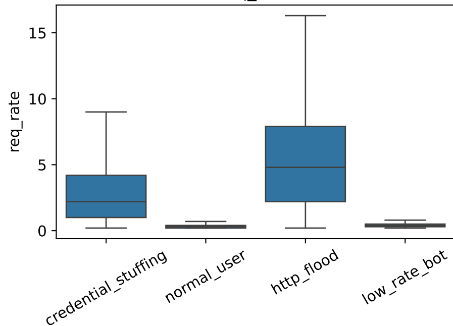
req_rate
