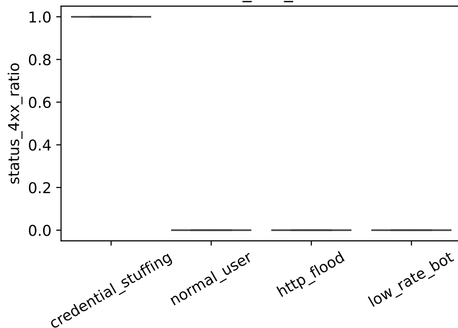
status_4xx_ratio
