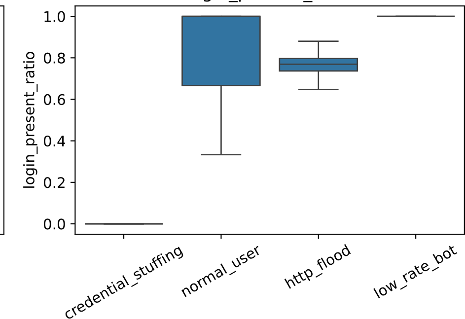
login_present_ratio
