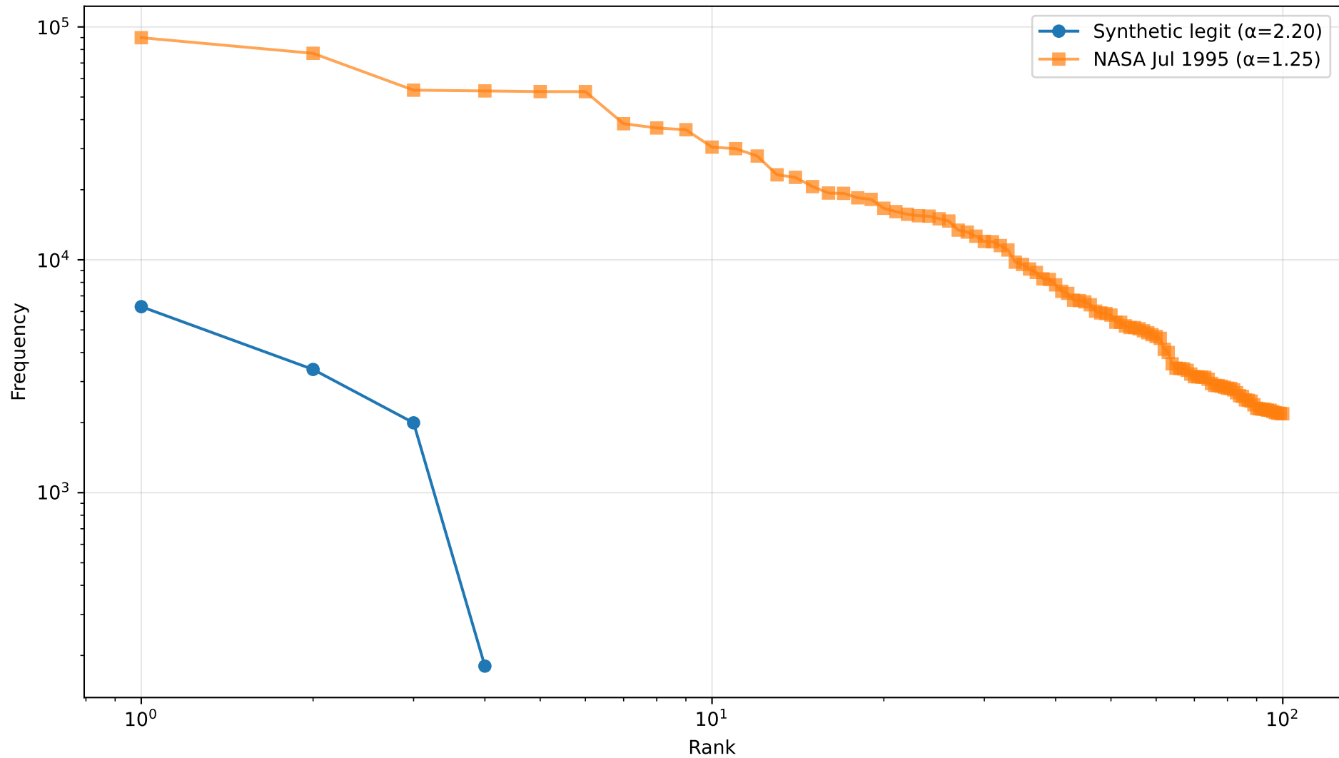
Endpoint popularity reference comparison — synthetic vs NASA
