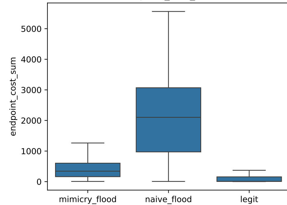
endpoint_cost_sum
