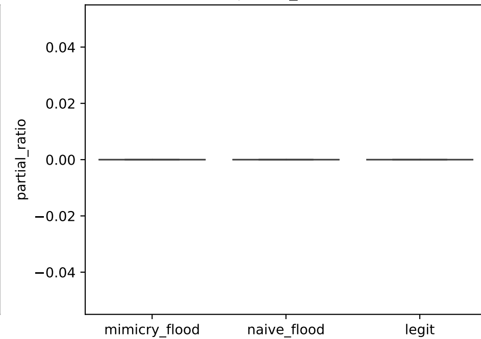
partial_ratio
