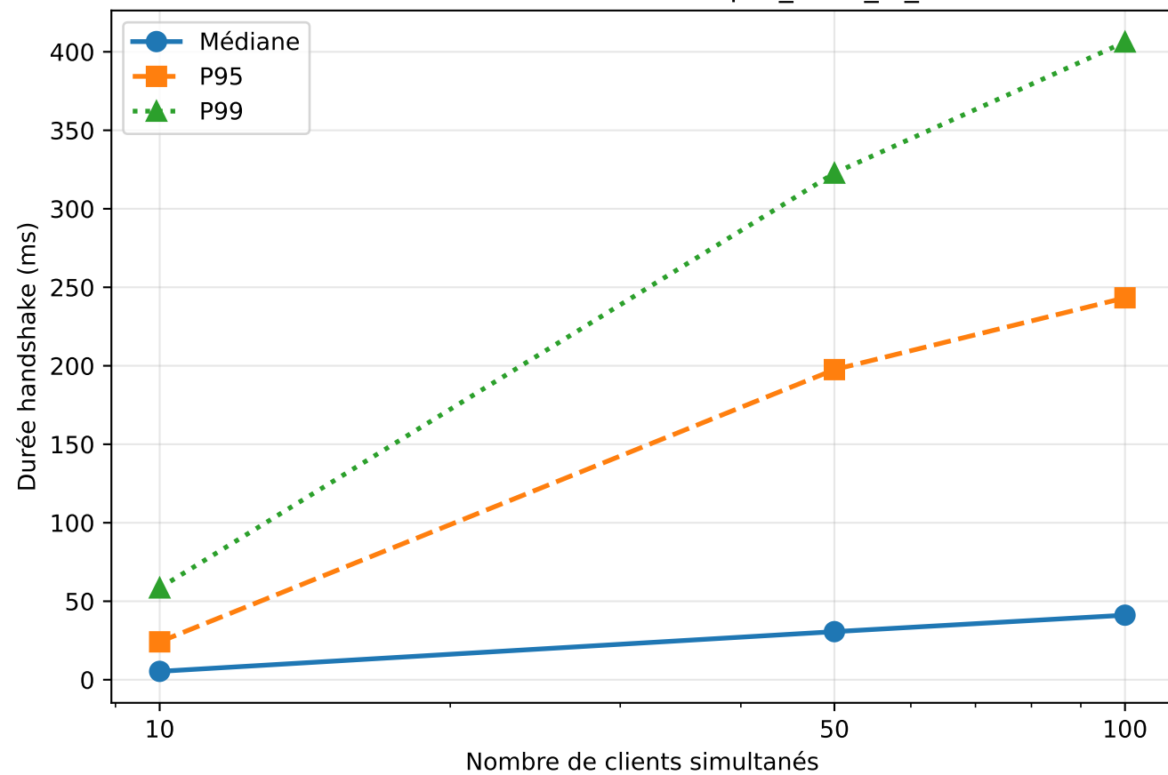
Latence vs Concurrency — quic_none_l0_d0
