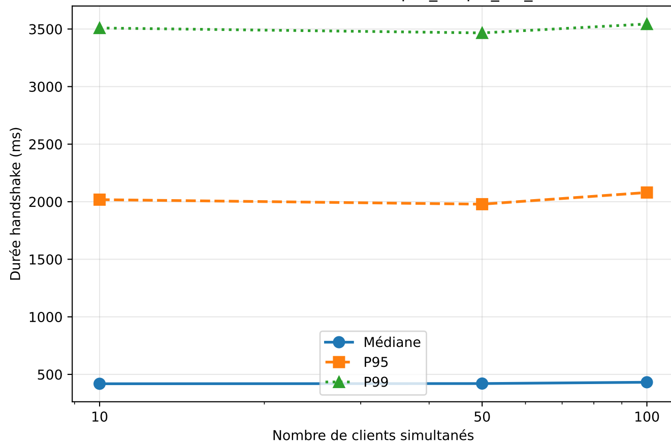
Latence vs Concurrency — quic_simple_l10_d200
