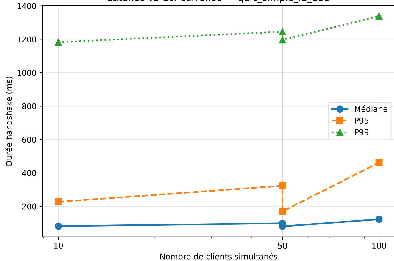
Latence vs Concurrency — quic_simple_l2_d35
