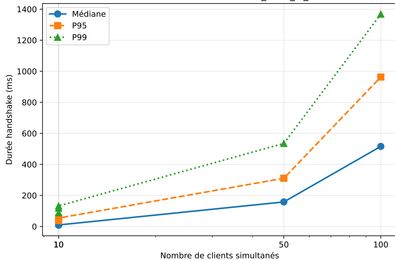
Latence vs Concurrency — tls_none_l0_d0
