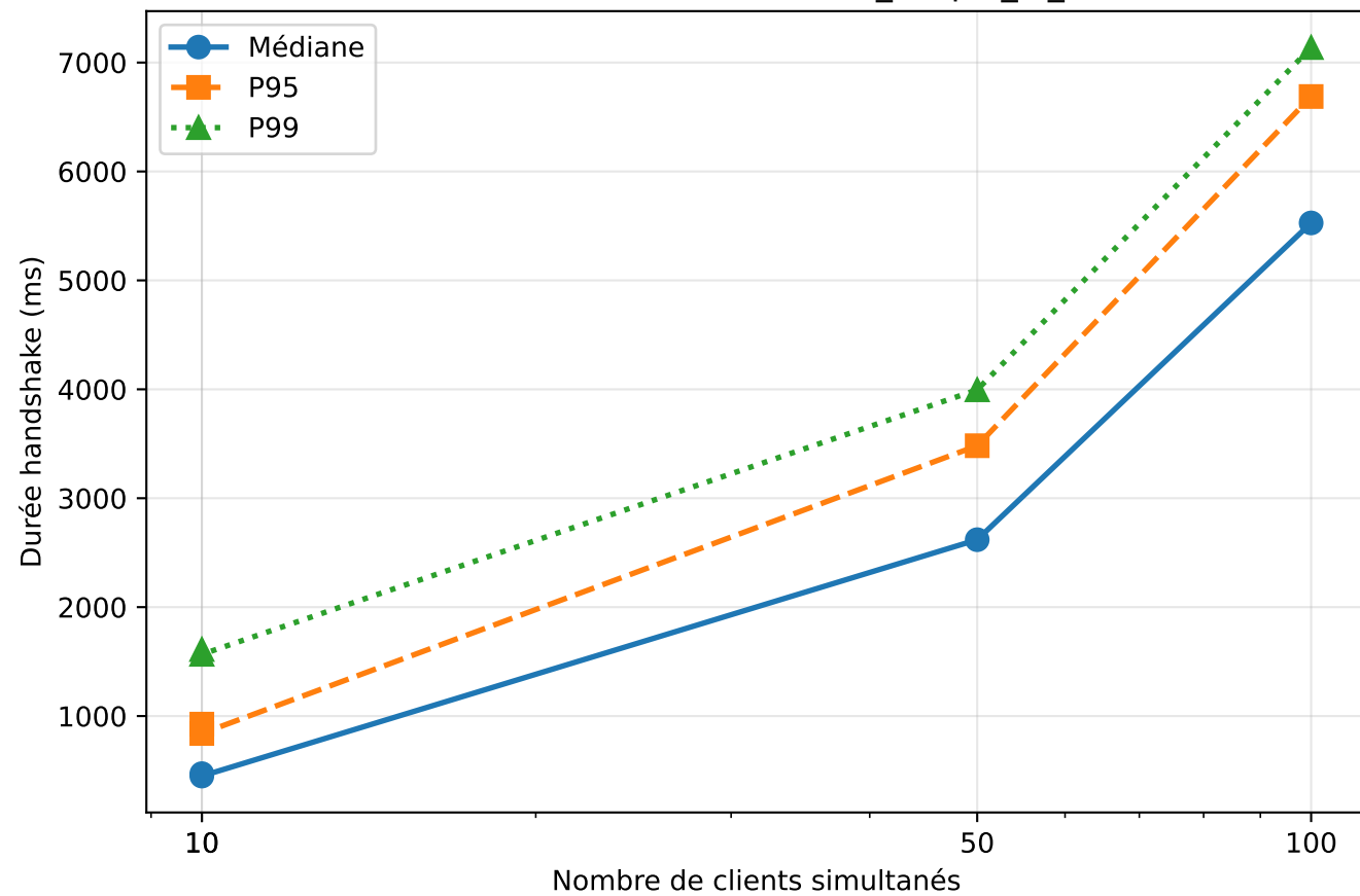
Latence vs Concurrency — tls_simple_l2_d35
