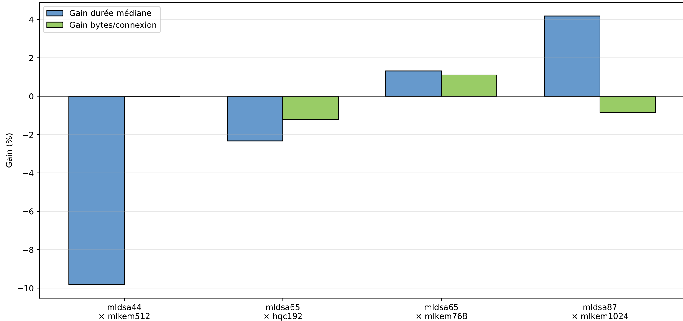
Impact compression certificat — QUIC (simple)
