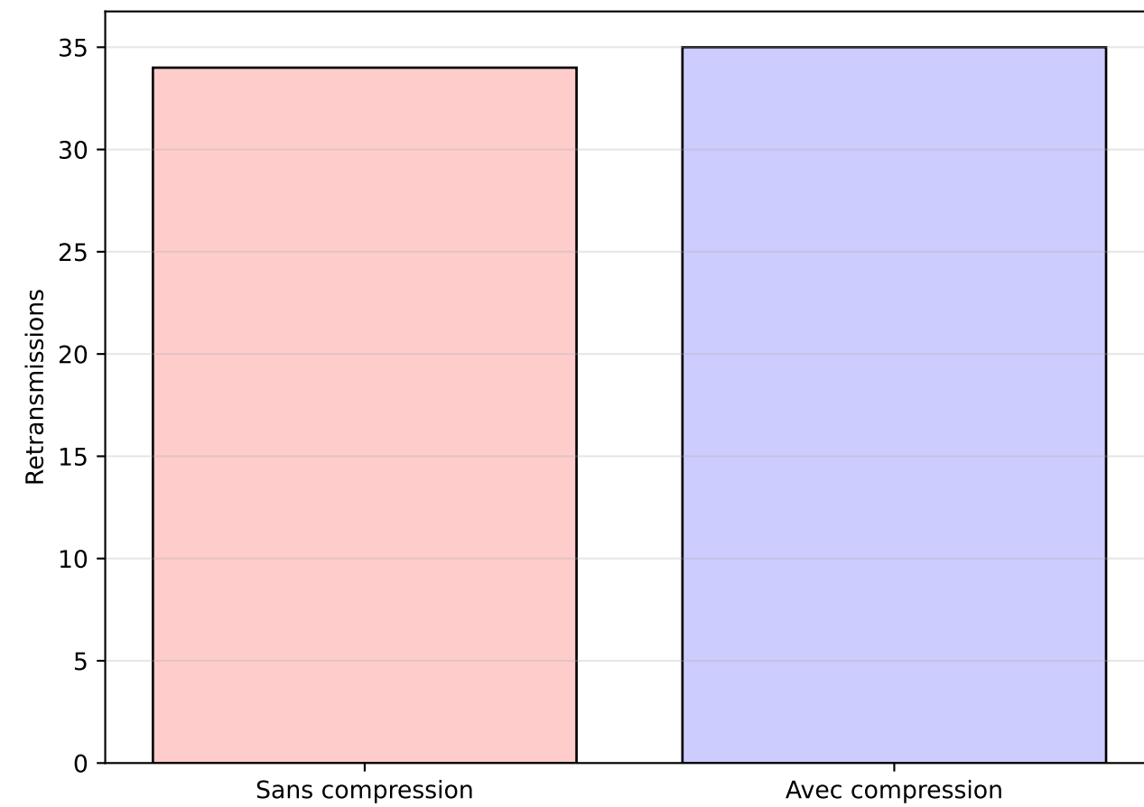
Retransmissions TCP
