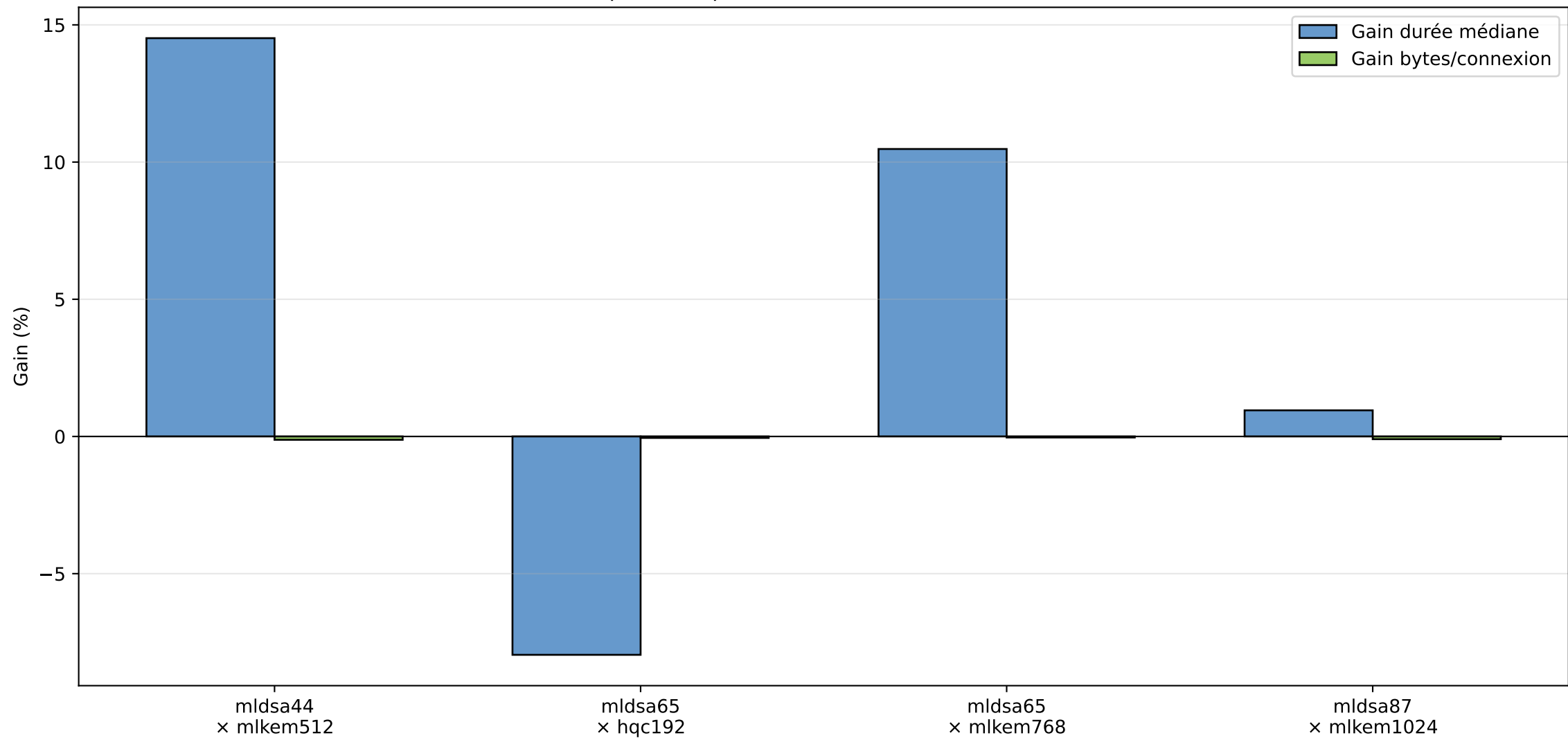
Impact compression certificat — TLS (none)
