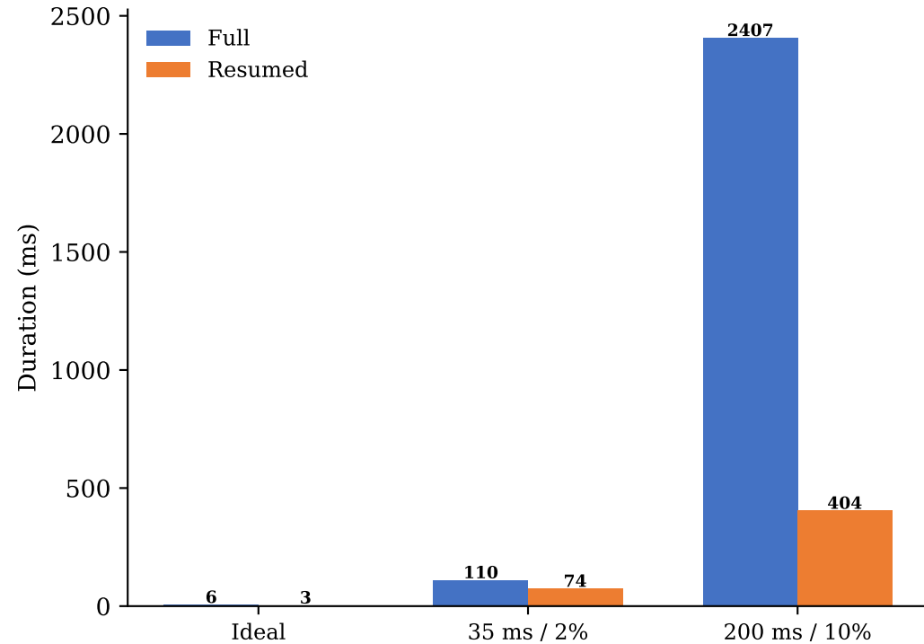
QUIC — Full vs Resumed
