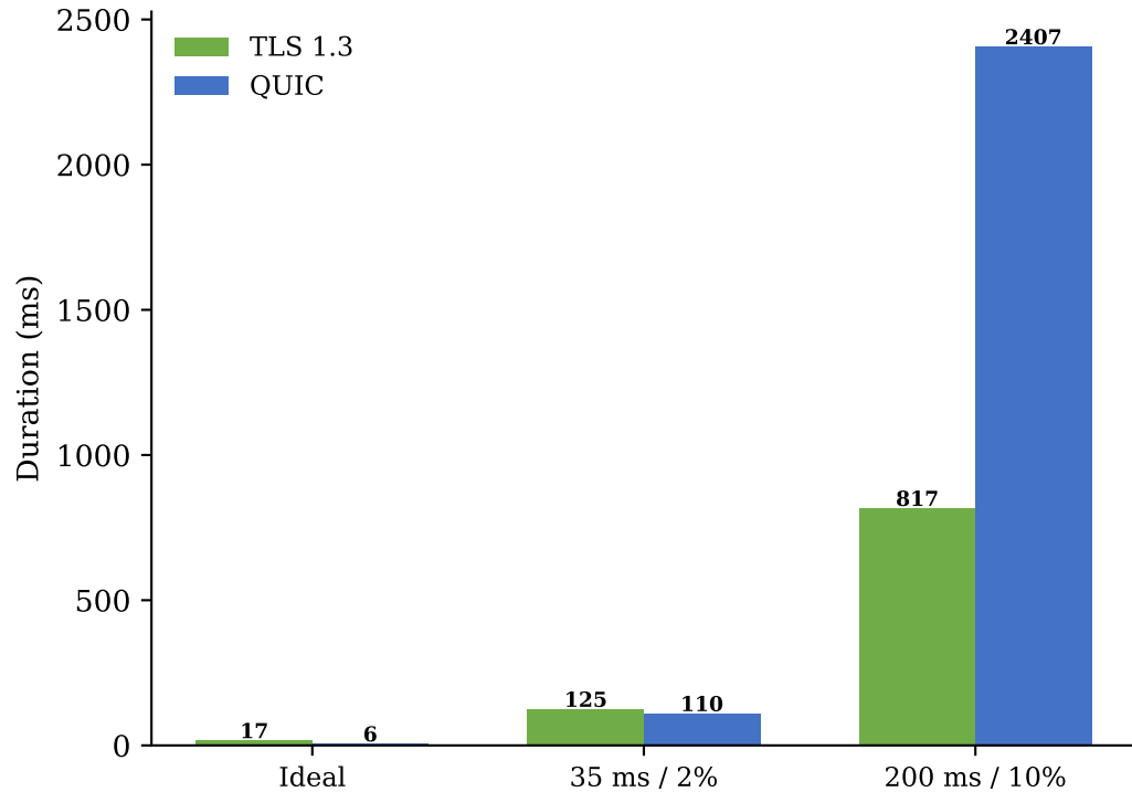
TLS 1.3 vs QUIC — Full Handshake
