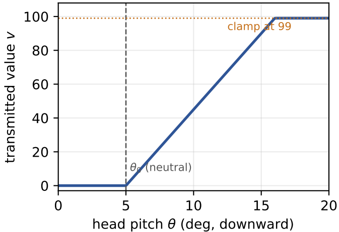
(a) angle to pedal value
