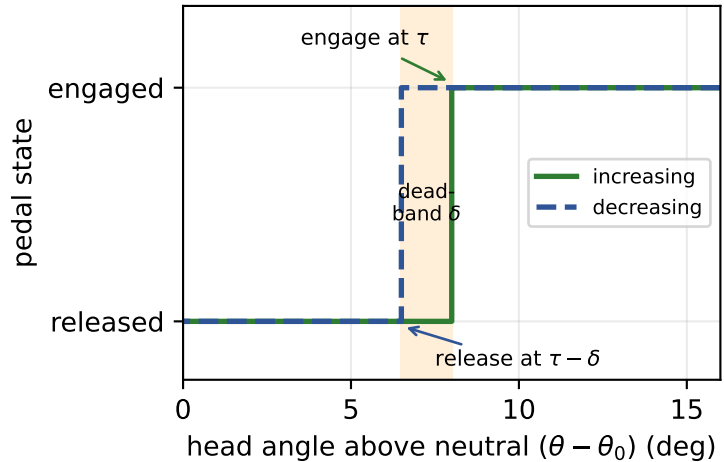
(b) engage/release hysteresis
