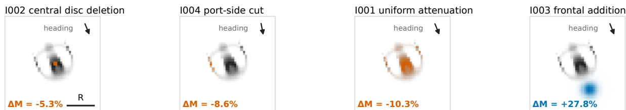
Figure A. Orbium (S001) survival boundary under four standardised disturbances
