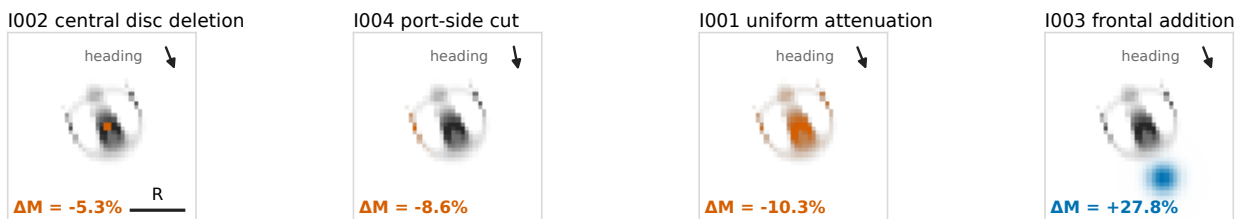
Figure A. Orbium (S001) survival boundary under four standardized disturbances
