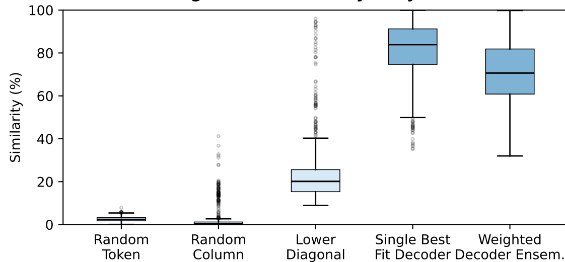
Program IoU Similarity: TinyLlama
