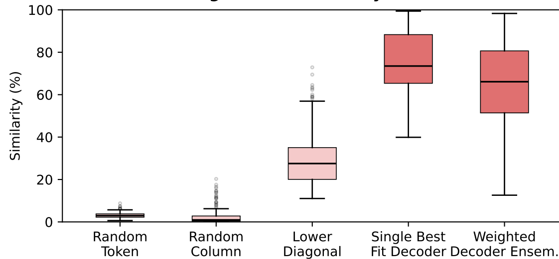
Program IoU Similarity: GPT-2
