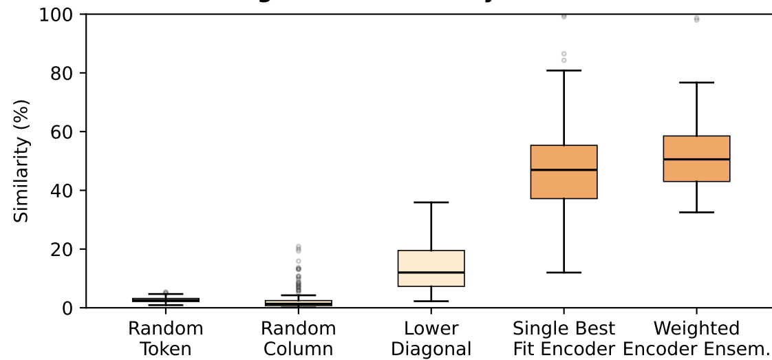
Program IoU Similarity: BERT-BASE
