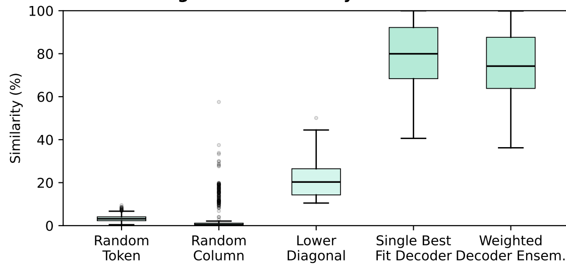
Program IoU Similarity: Llama-3.2-3B
