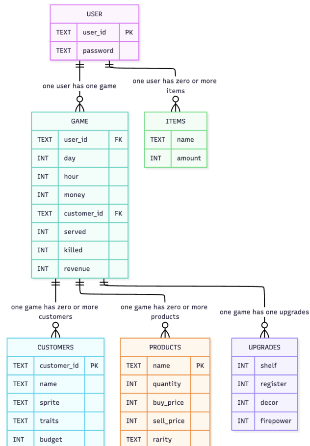
Figure 3: Database Algorithm
