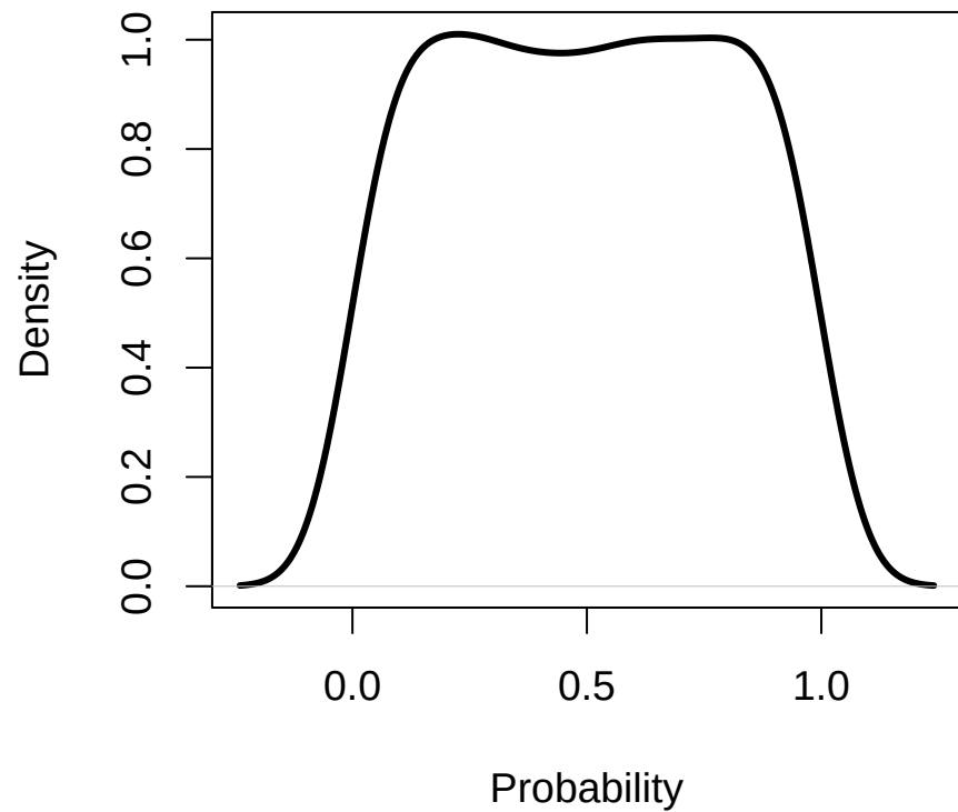
probability-scale
