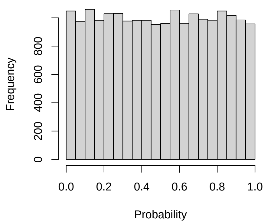
probability-scale
