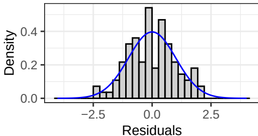
Histogram
