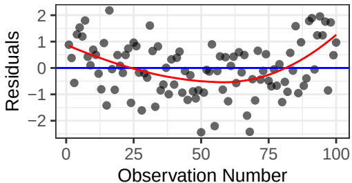
Index Plot
