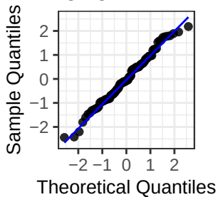
Q-Q Plot
