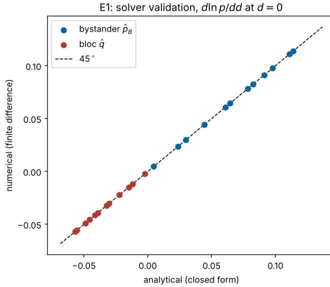
Figure 1: Solver validation. Numerically computed price responses plotted against their closed-form counterparts at d = 0 , for bystander (disruptor) and bloc goods. Each dot corresponds to one of twelve (\sigma, \tau_0) calibrations, with the 45-degree line superimposed. Maximum absolute error is 9 \times 10^{-8} .
