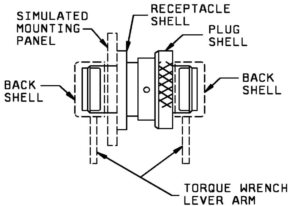
FIGURE 23. Rear accessory thread strength test.
