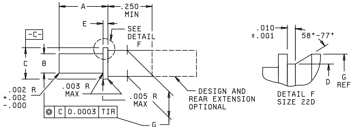
SIZE 12 THROUGH 22
