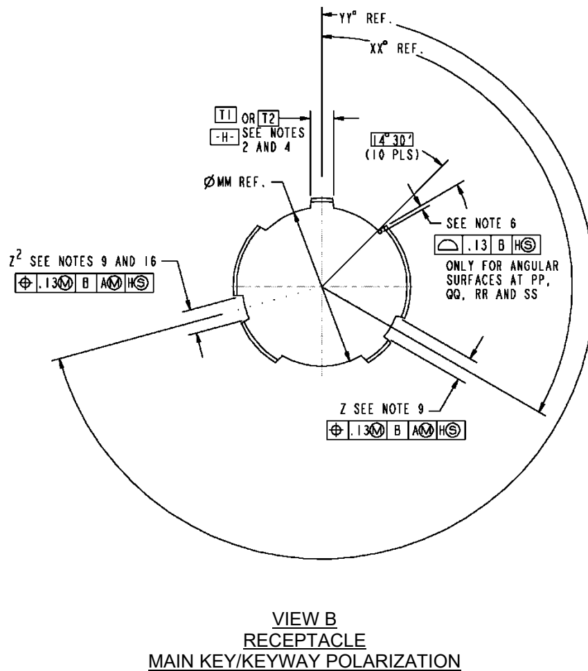
FIGURE 7. Connector intermateability dimensions (series IV), Main key / keyway polarization - Continued.
