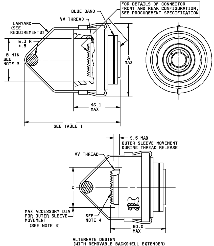
FIGURE 1. Plug.
