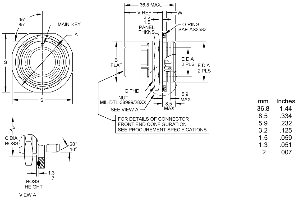
FIGURE 1. Receptacle, classes N and Y.
