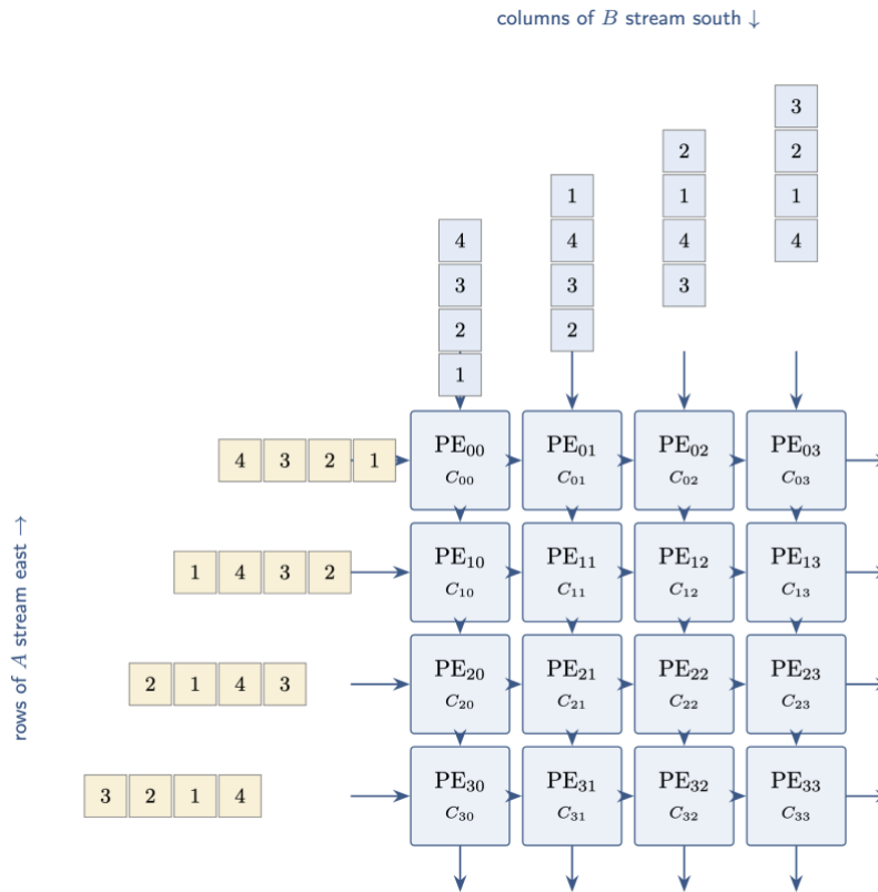
Figure 4. 4 \times 4 Output-Stationary Systolic Array
