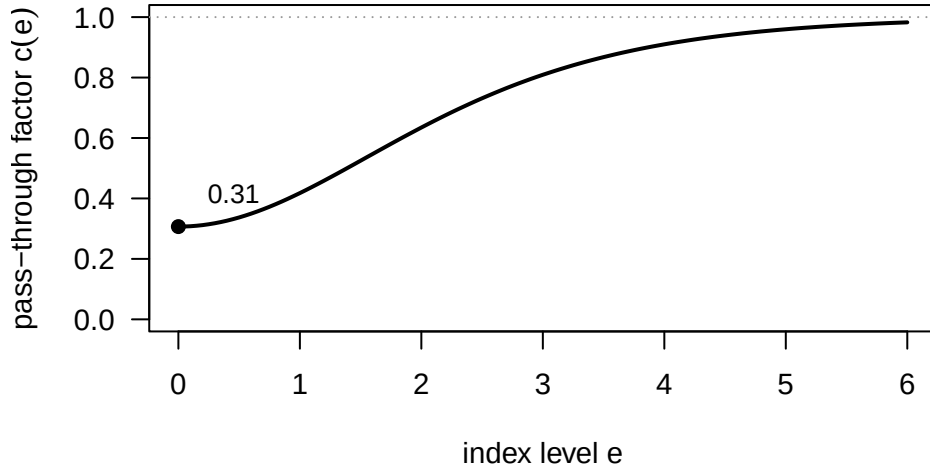
Figure 2: Pass-through factor c(e) under a logistic link. Imputation-model error at signal level e reaches \hat{\theta} multiplied by c(e) , which climbs from about 0.31 at e = 0 toward 1 as the signal grows: the truncation self-corrects when Y is informative and stops doing so once Y is near-deterministic. Averaging c over the index distribution gives the \bar{c}_1 quoted in the text.
