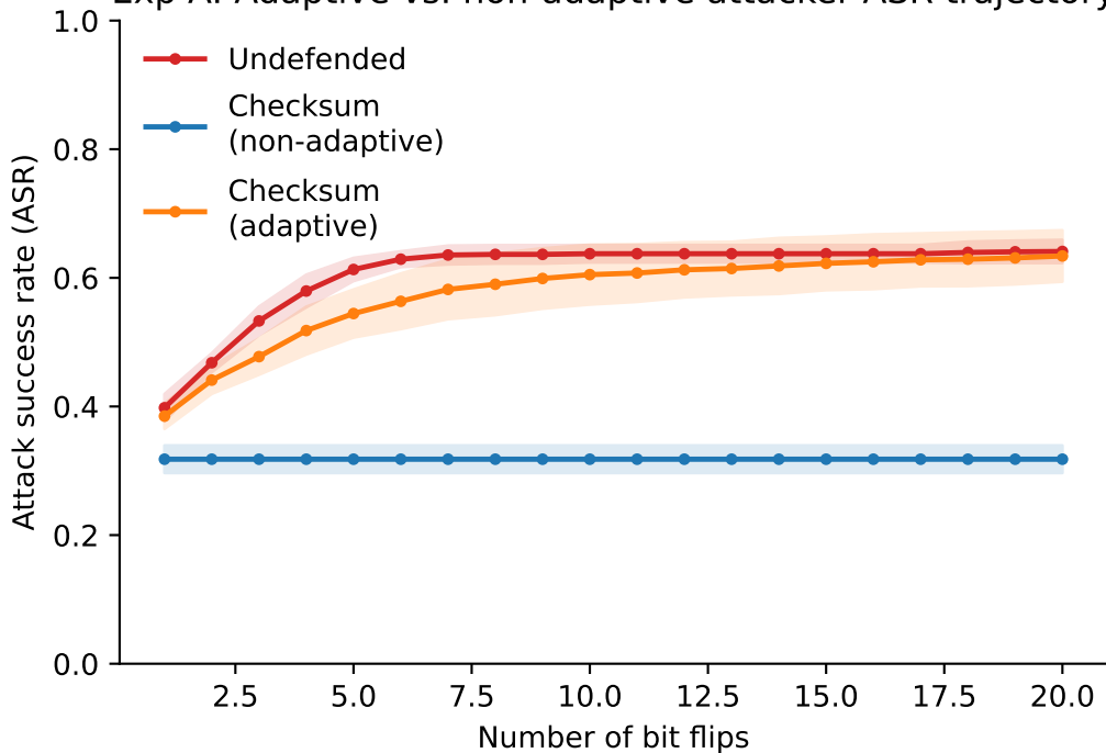
Exp A: Adaptive vs. non-adaptive attacker ASR trajectory
