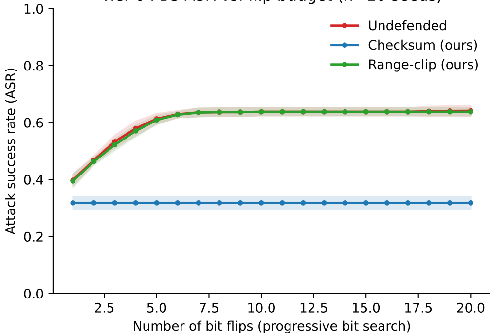
Tier-0 PBS ASR vs. flip budget (n=10 seeds)
