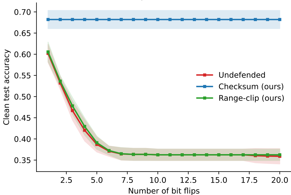
Clean-accuracy retention under attack
