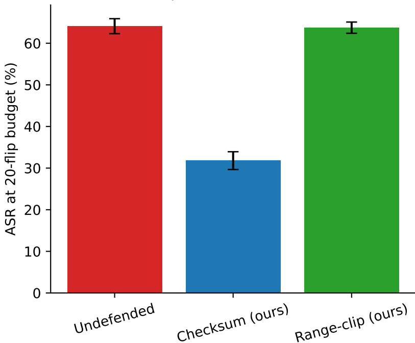
Defense comparison, Tier 0 (n=10 seeds)
