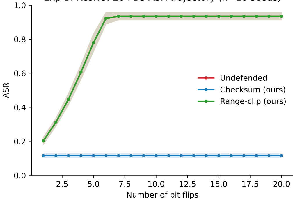
Exp B: ResNet-20 PBS ASR trajectory (n=10 seeds)
