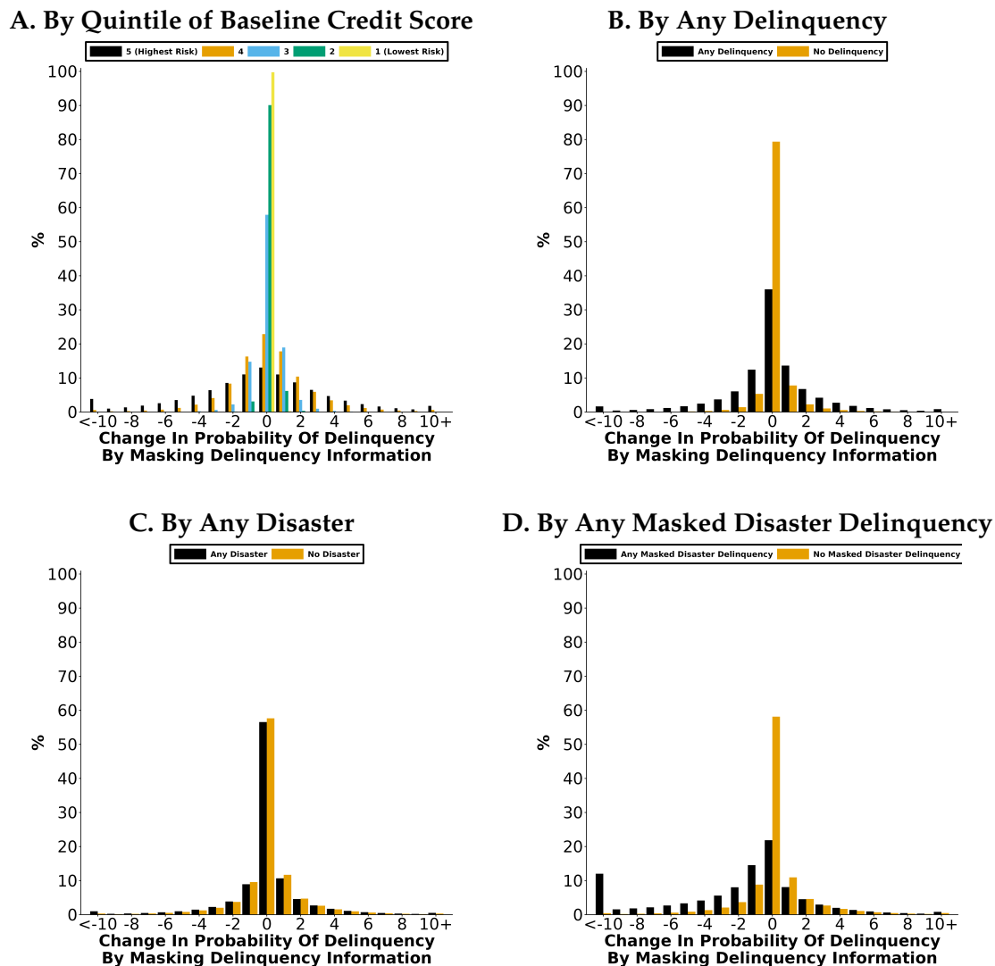
Figure 8: Distribution Of Percentage Point Changes In Probability Of Delinquency, Calculated For CARES Model Masking Of Disaster Delinquency Information For Three Months, Relative To Baseline Model With Delinquency Information
