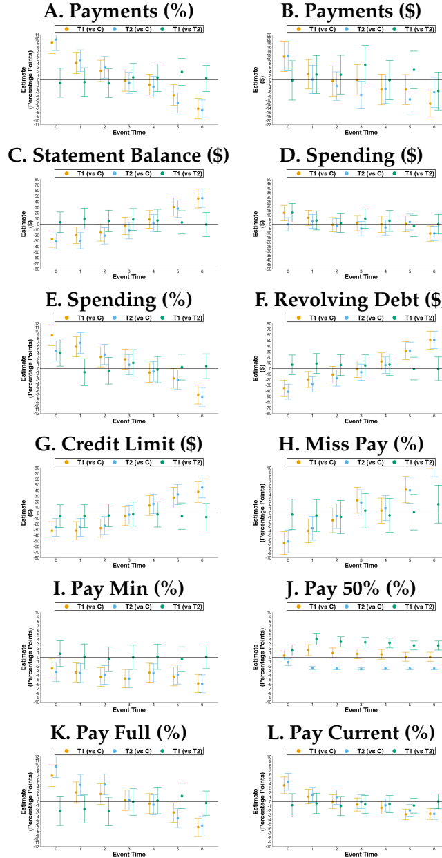
Figure A4: Dynamic Effects On Primary And Secondary Outcomes, No Time F.E.
