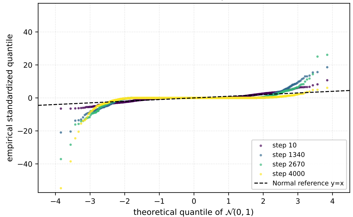
(b) Normal Q-Q plot
