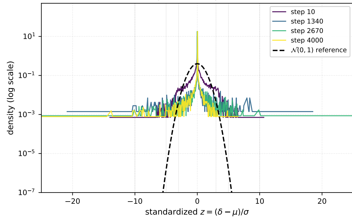
(a) Empirical density vs \mathcal{N}(0, 1)
