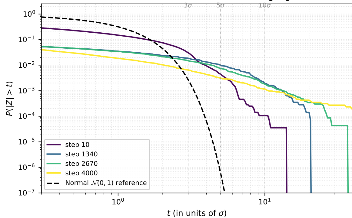
(c) Tail survival function vs Normal (log-log)
